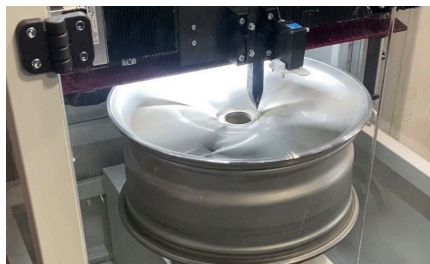
LATHE
